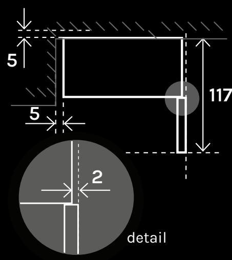
Doors opening dimensions (cm)
